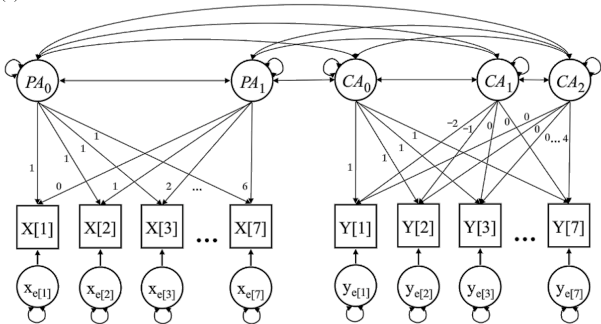
Figure 1. (a) Linear latent growth curve model of positive affect (PA). (b) Bivariate piecewise latent growth curve model of positive affect (PA) and cognitive ability (CA). Although not depicted in panel b, means for the growth factors are estimated. For clarity, parameters are not labeled in panel b.
